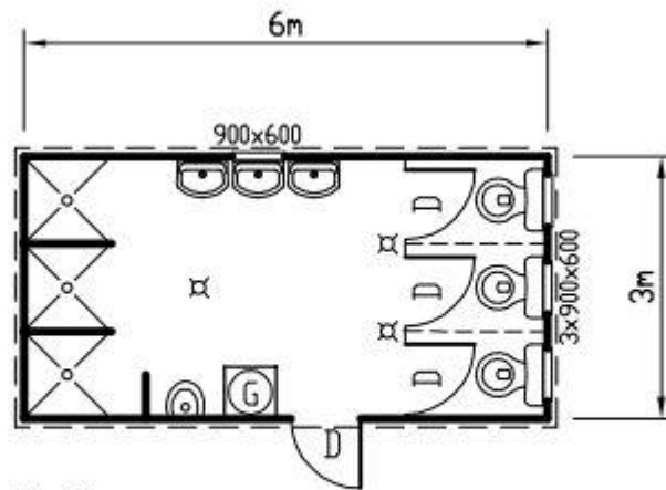
PLAN 18m 2
